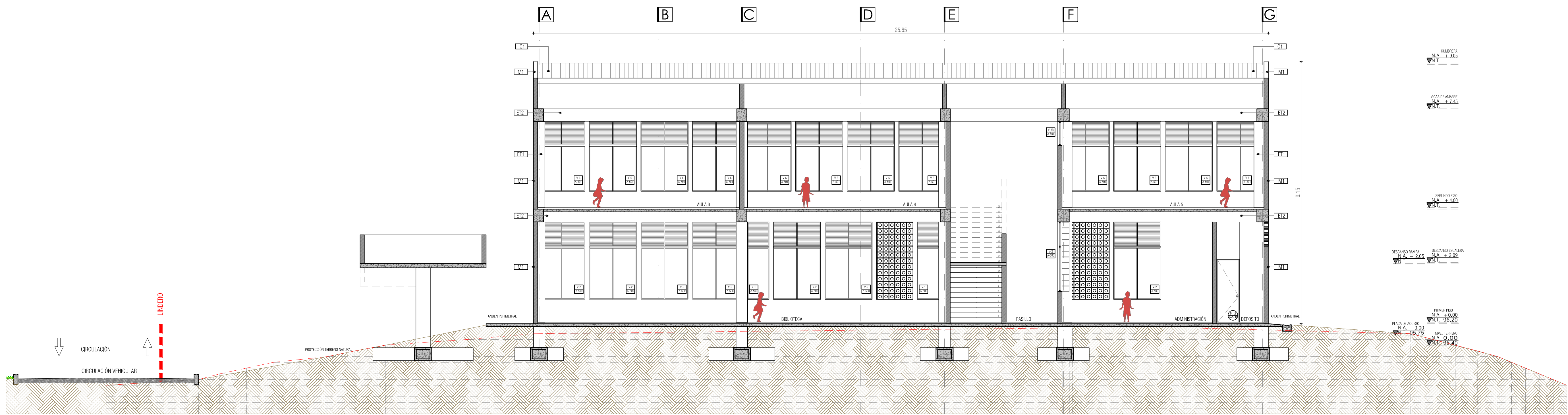
I.E. AGROECOL SAN RAFAEL CHOCO CORTE GENERAL 1 ESC 1_75
