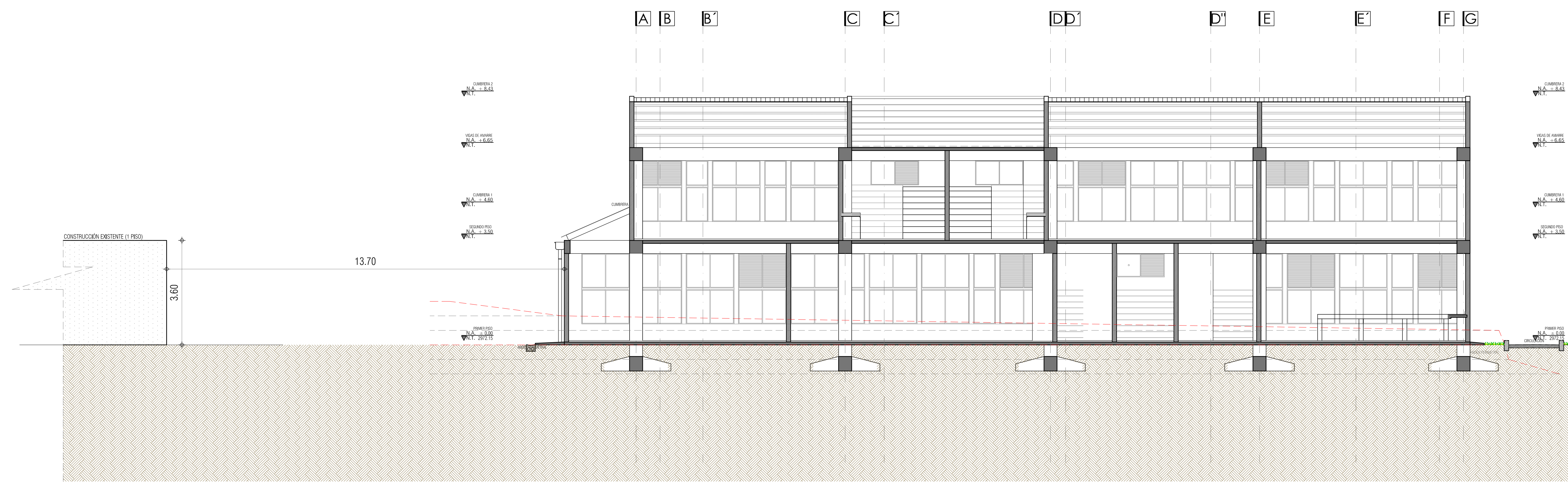
IE SOCORRO CIMARRONES CORTE GENERAL 1 ESC 1_75
