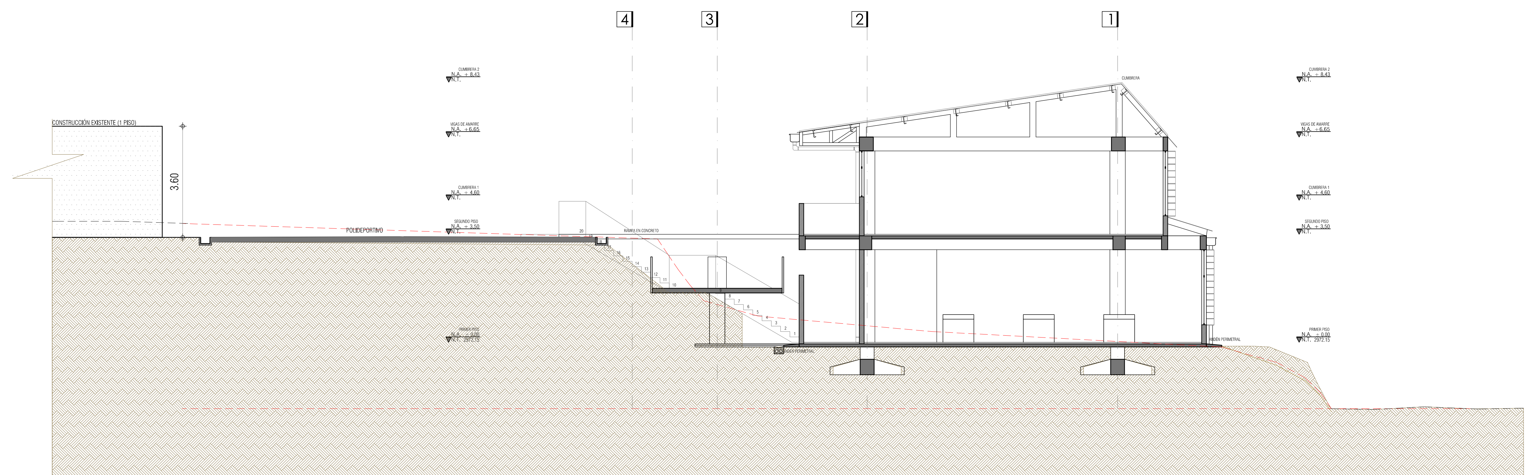
IE SOCORRO CIMARRONES CORTE GENERAL 2 ESC 1_75
