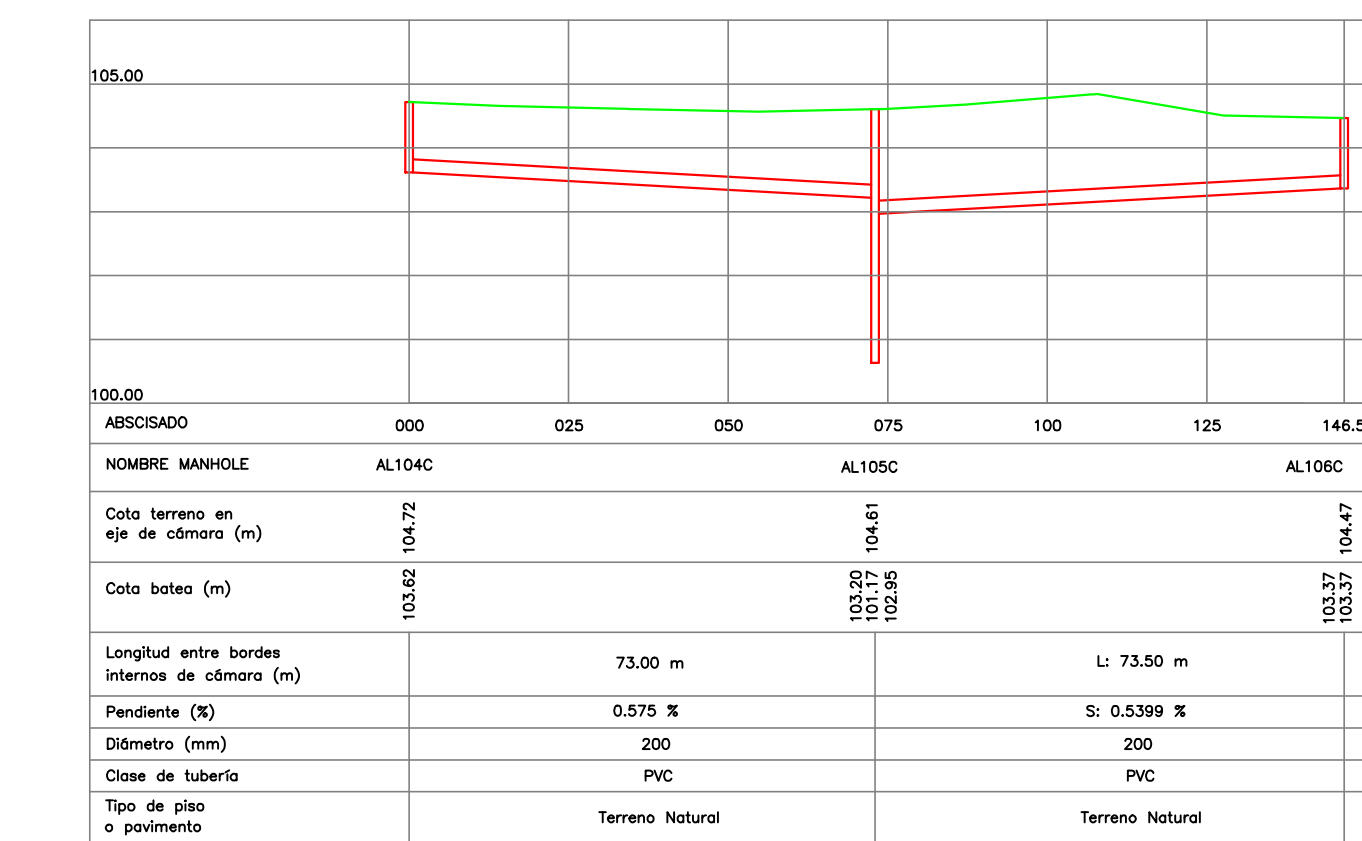
PERFIL MANHOLES AL104C - AL106C
