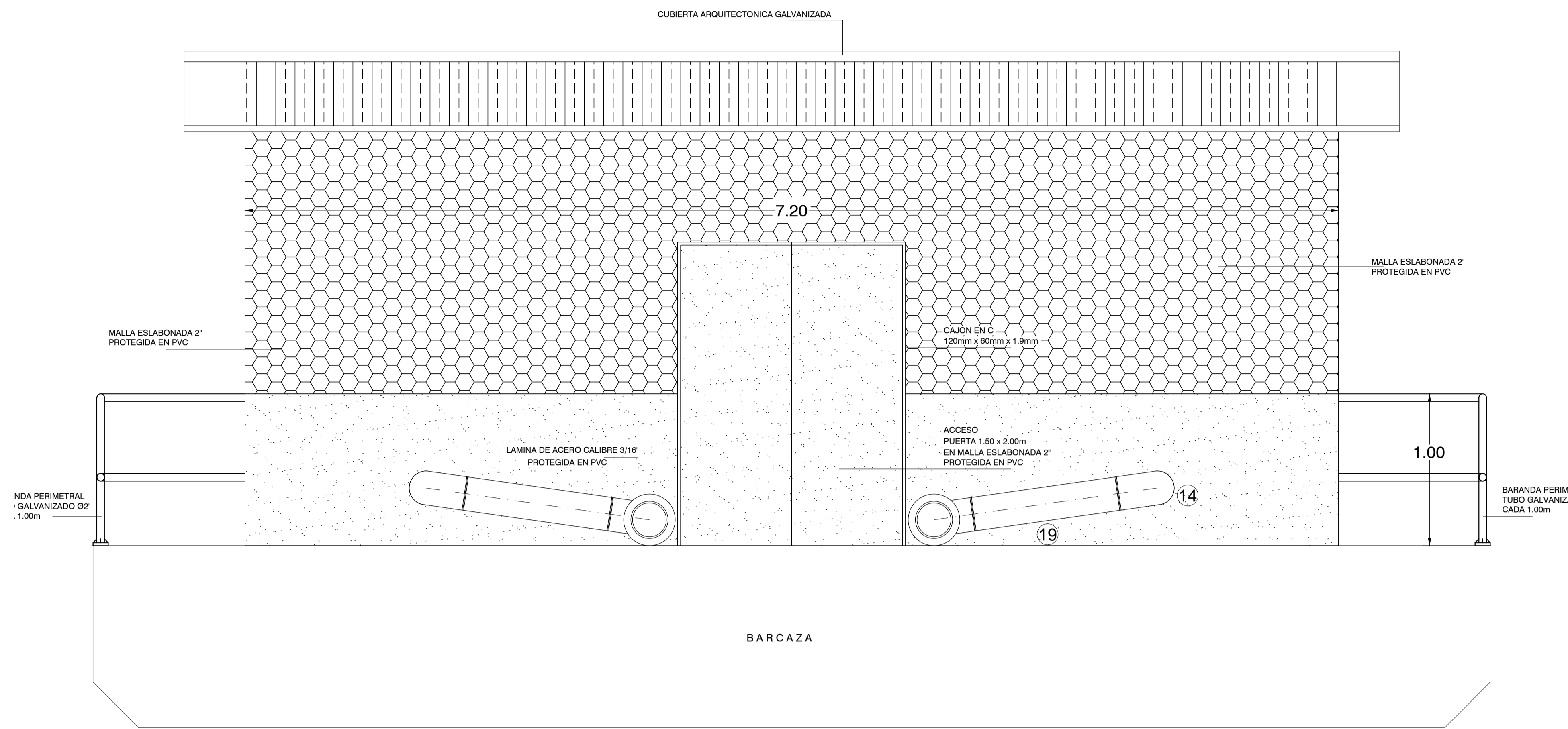
FACHADA PRINCIPAL ESC: 1:20
